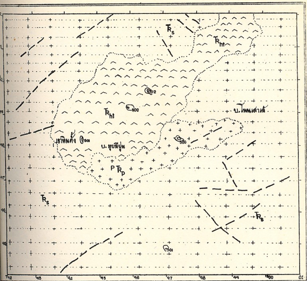
Geologic Map of Ban Yup E-poon and Ban Non Sao Ae Area After Chaiyan Hin Thong, 1976 Geologic map Sheet 47P/FG 11 and 47 P/ FG 12
