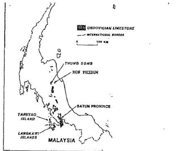
Figure 2 Map showing the location of areas mentioned in the text and the distribution of Ordovician strata in Thailand and Malaysia.
