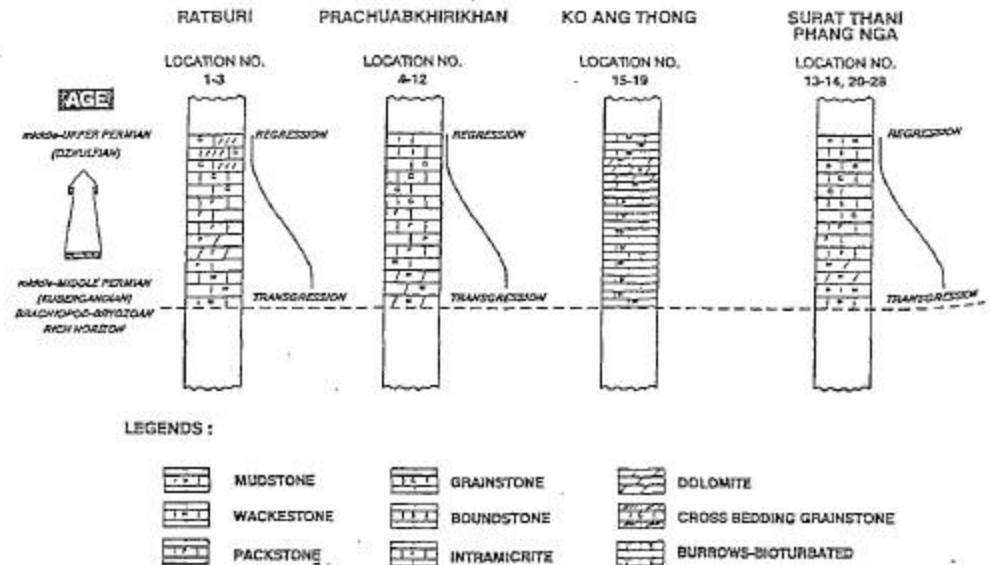
Fig. 6. Facies interpretation of Permian carbonate section in southern Thailand. Location no. refer to sample locations map in the text (Not to scale.) (After Chinoroje, O., 1993)
